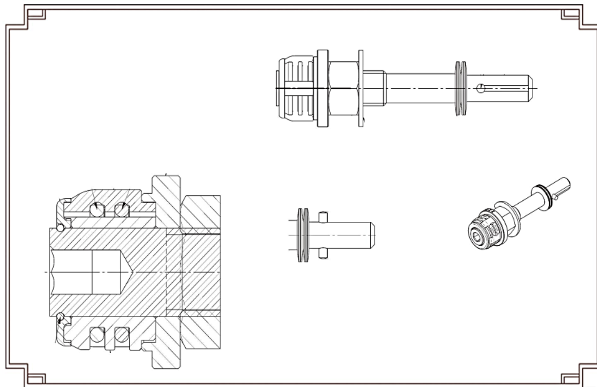
Spare part number: 0902673864 Replacement number: SD/2673867 Name: mandrel head
